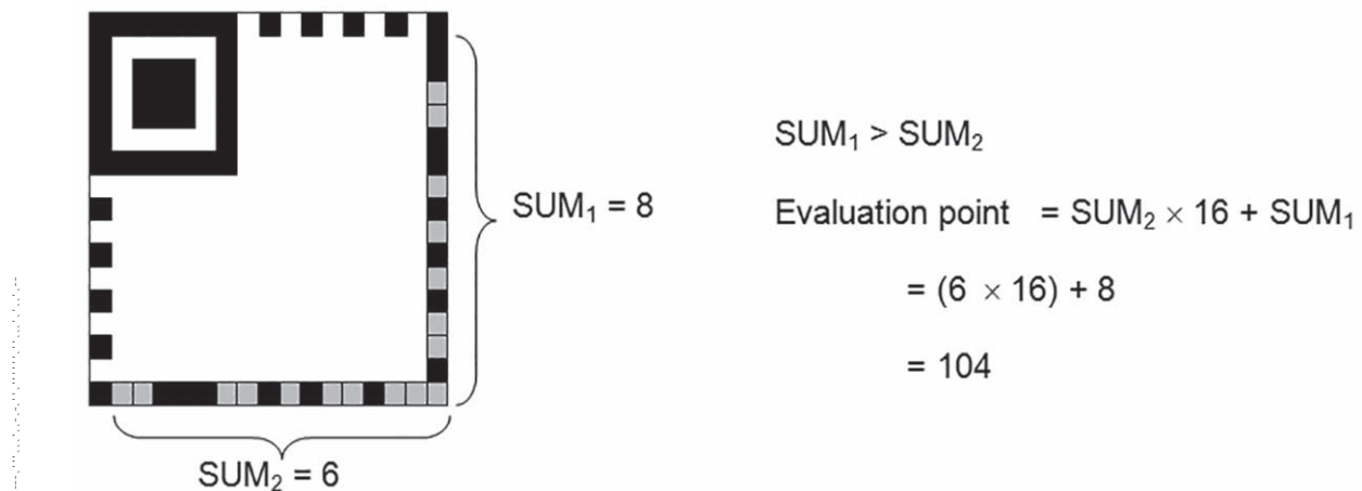
Figure 24 — Evaluation of masking results in Micro QR Code symbol
